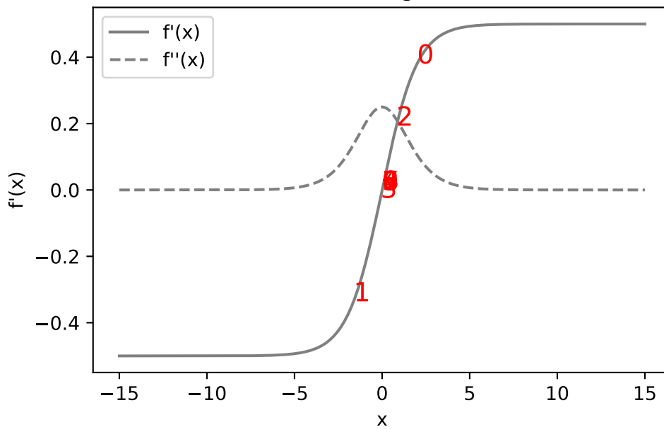
converges
