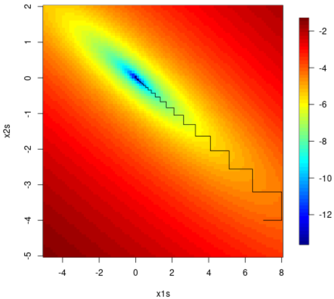
Figure 2: Coordinate descent
